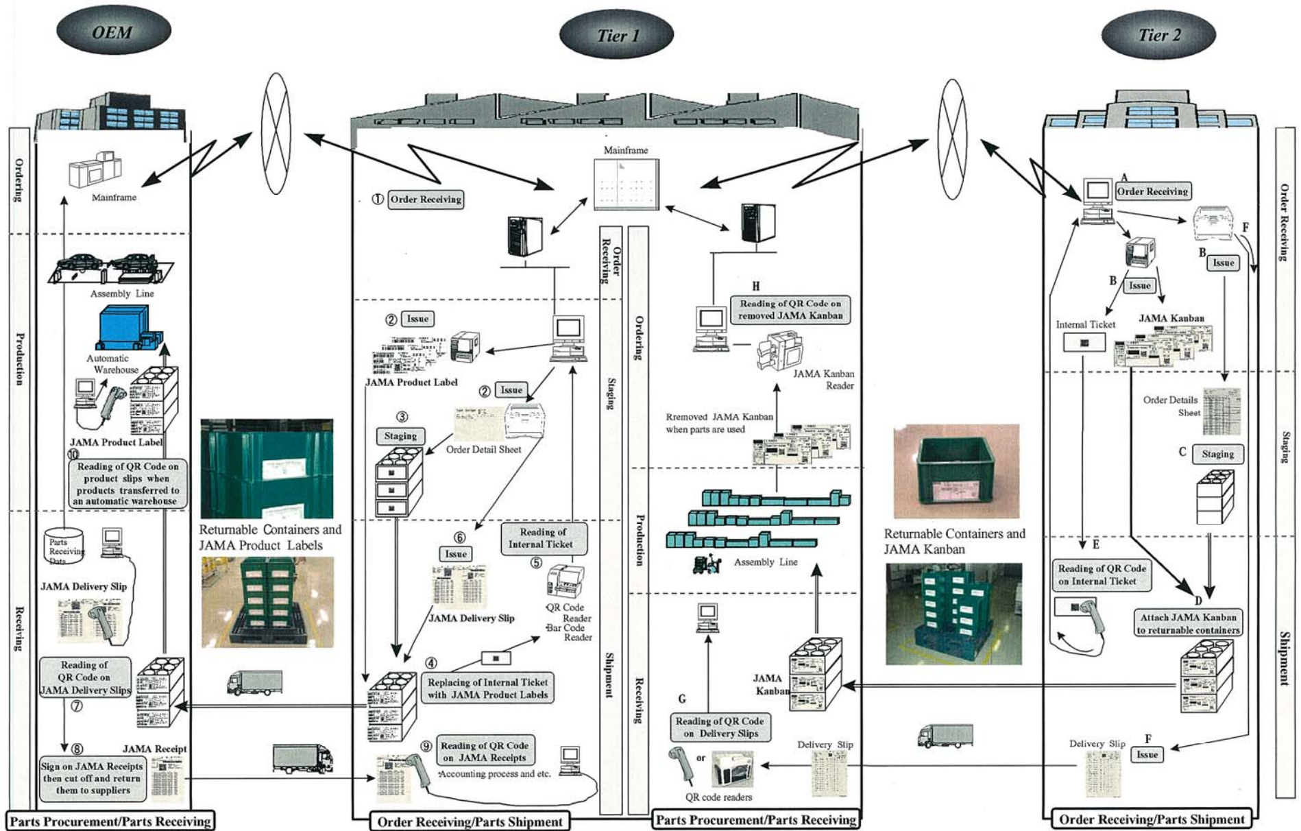
Example of process flow with JAMA standard Shipping Label (Domestic procurement)
